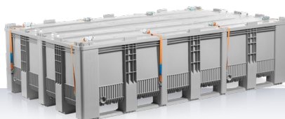
SB | 2988 L 50H/Y/.../D/BAM 16293-CTP/2630/1383 ① 2950 x 1850 x 790 mm ② 2965 x 1863 x 862 mm Max. gross weight: 1383 kg Standard colours: ■
