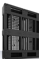
D3/D3-5 1200 × 1000 × 150 mm Standard colours: ■
